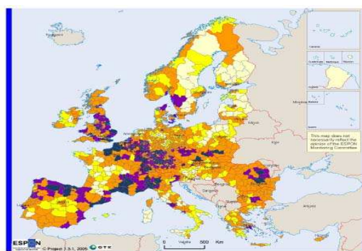
Map 1. Aggregated hazards
